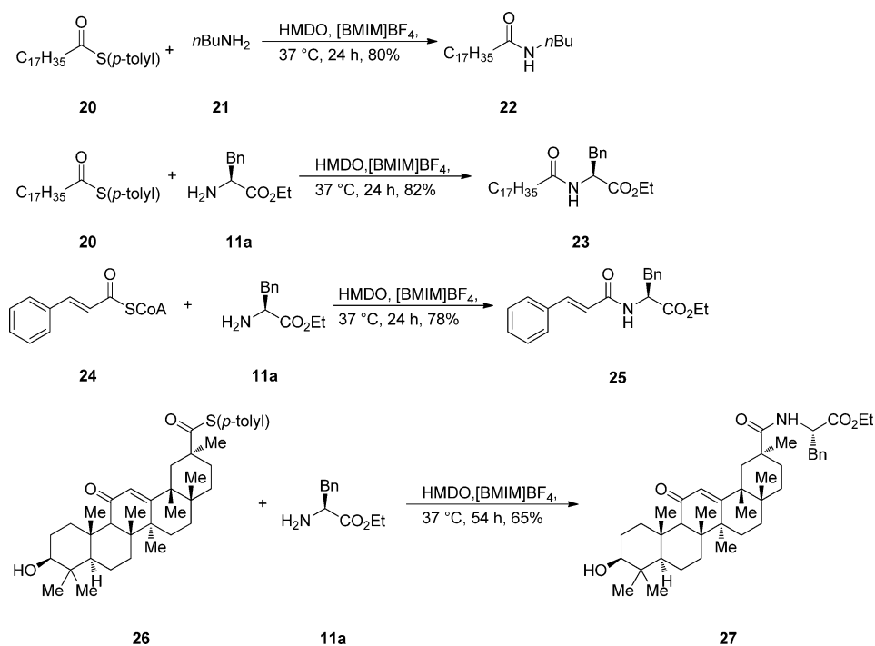
Scheme 5. Proposed Approach for Lysozyme Modification
