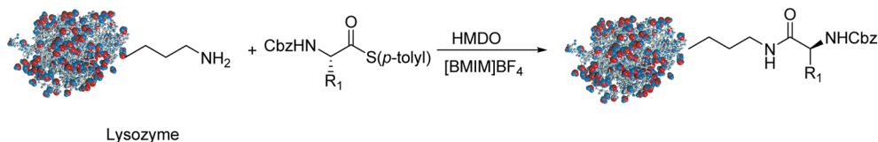
Scheme 5. Proposed Approach for Lysozyme Modification
