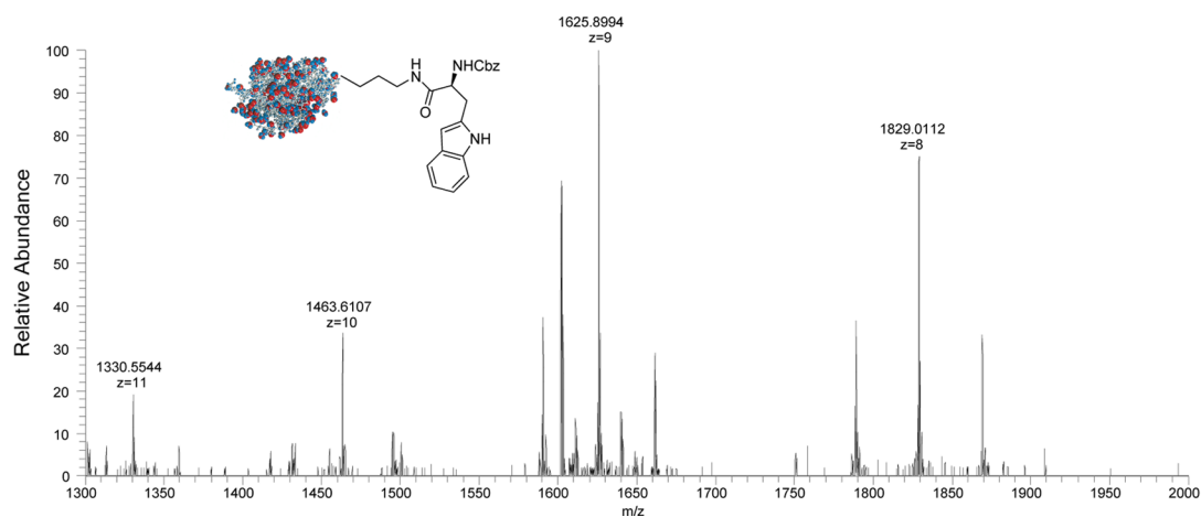
Figure 1. LTQ Orbitrap XL-MS spectrum of the lysozyme (A), N-Cbz-L-Phe-lysozyme (28) (B), and N-Cbz-L-Trp-lysozyme (29) (C).
